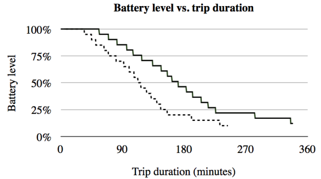
Fig. 3: The push-based policy recalculation provides a significant power savings to the user. In a “periodic refresh” scenario, shown by the dashed line, the battery completely discharges after a 4-hour trip. The “single download” scenario, shown by the solid line, is enabled by the existence of a push server, and enables the battery to last nearly 5.5 hours before full depletion, a 37% improvement.
